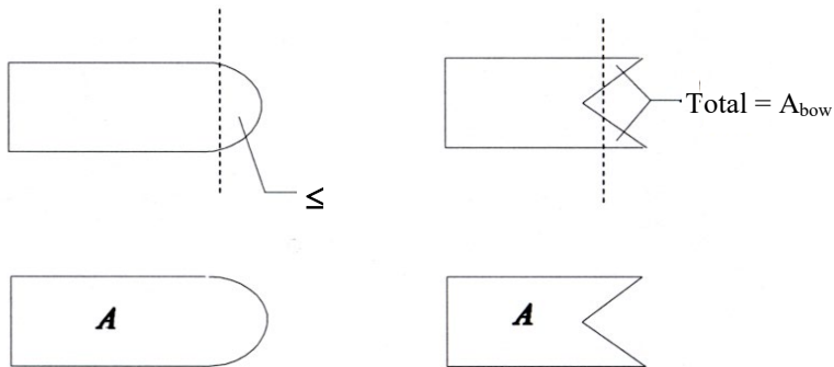
Figure 4.4.1: Plan view of two different craft styles
