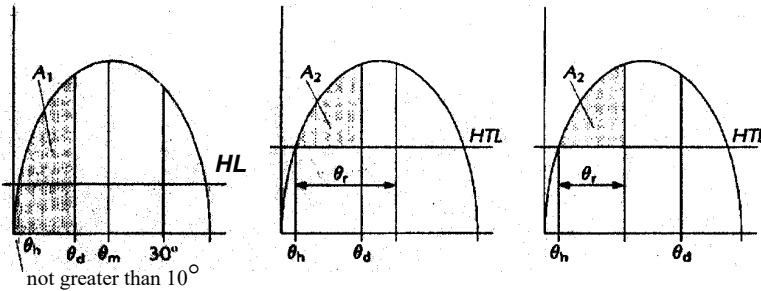
Figure 1 - Intact stability
