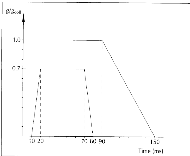
Figure - Acceleration time-history envelope
