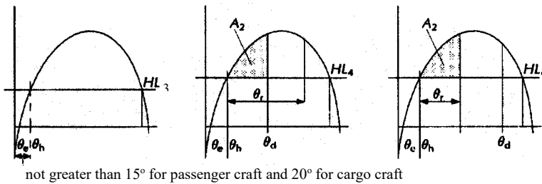
Figure 2 - Damage stability
